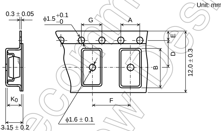
Figure 2 Tape Forms
