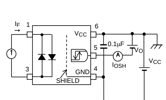
TEST CIRCUIT 6: I_{OSH}
