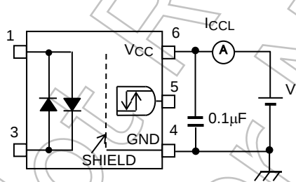
TEST CIRCUIT 3: I_{CCL}
