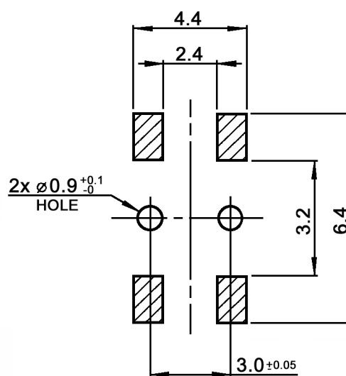
P.C.B. MOUNTING
