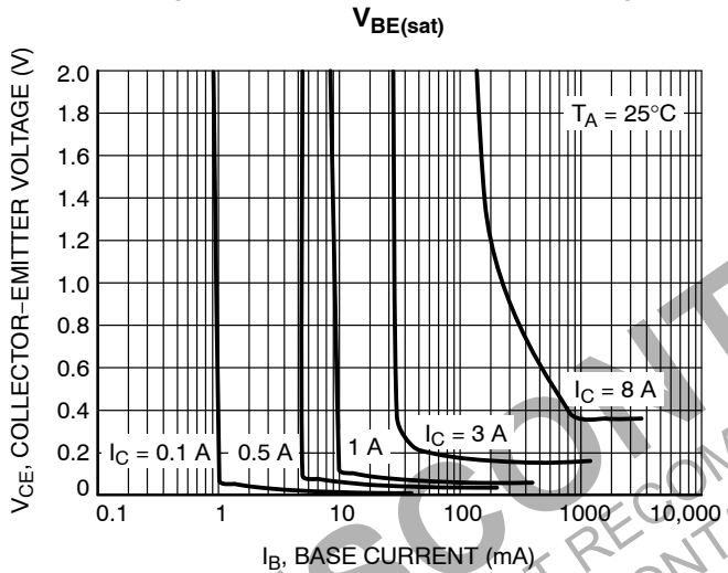
Figure 12. MJD44H11 Collector Saturation Region
