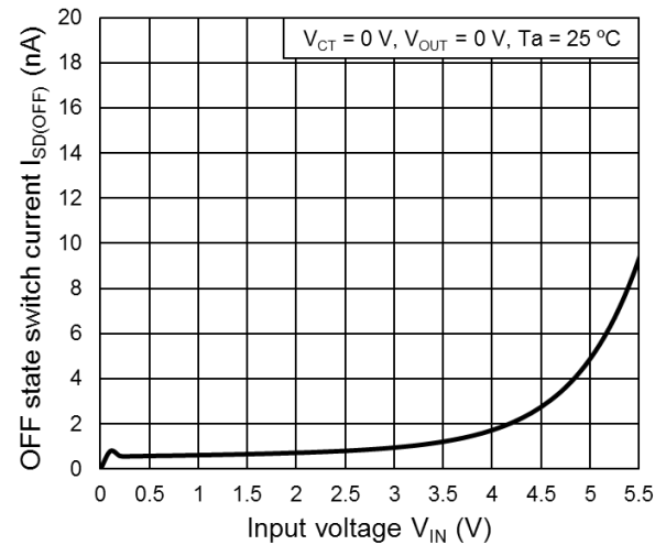
I_{SD(OFF)} - V_{IN}
