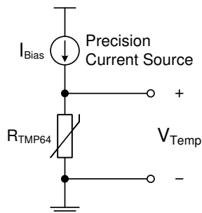
Figure 9-3. TMP64-Q1 Biasing Circuit With Current Source
