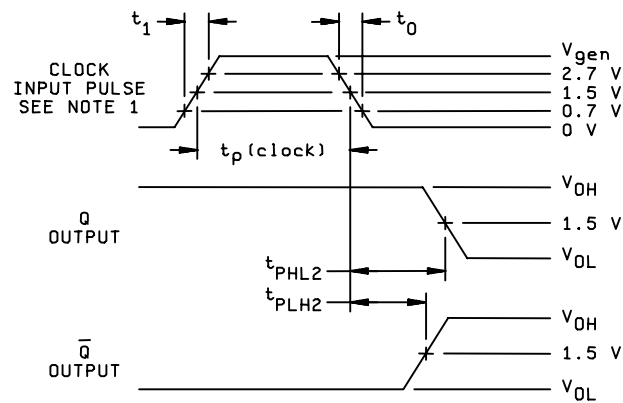
VOLTAGE WAVEFORMS
