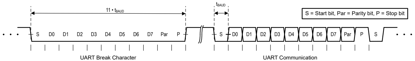
Figure 5-2. UBM Timing
