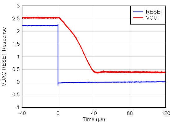
Figure 5-25. DAC RESET Response
