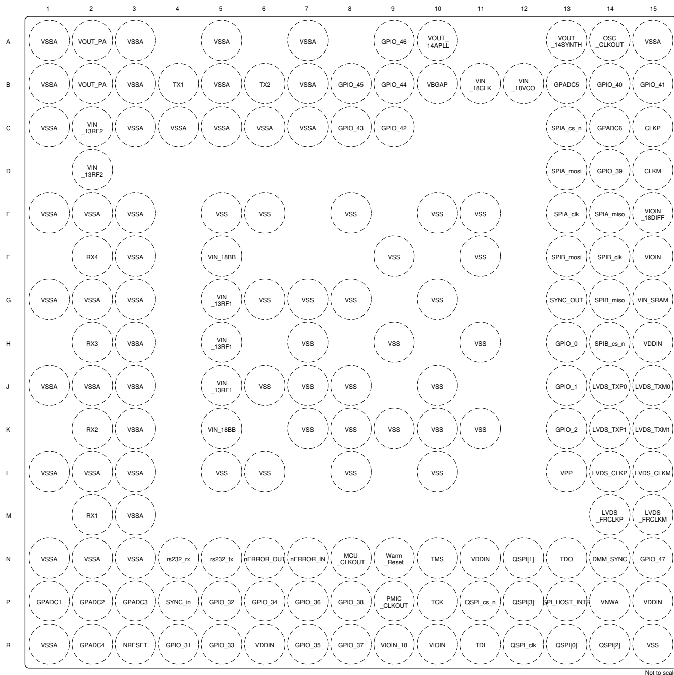
Figure 7-1. Pin Diagram
