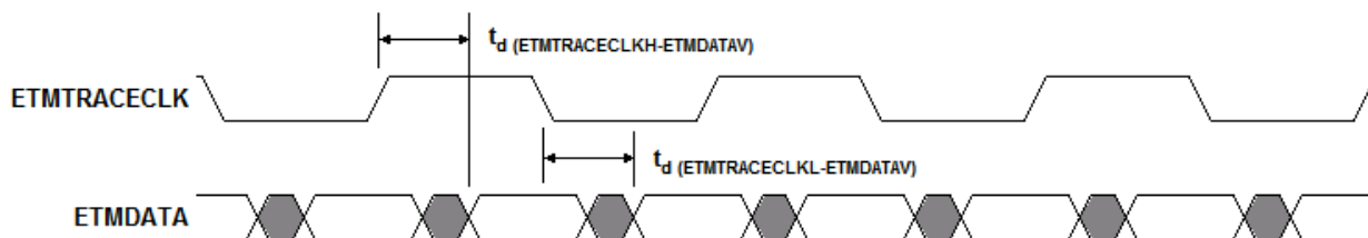
Figure 8-17. ETMDATA Timing
