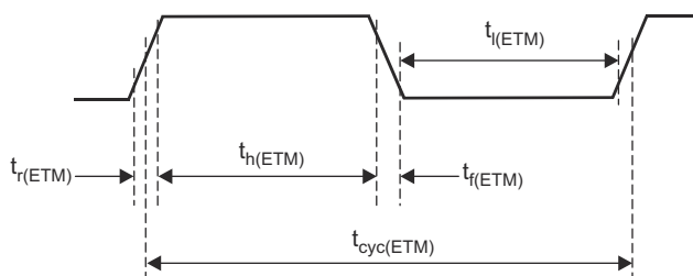
Figure 8-16. ETMTRACECLKOUT Timing
