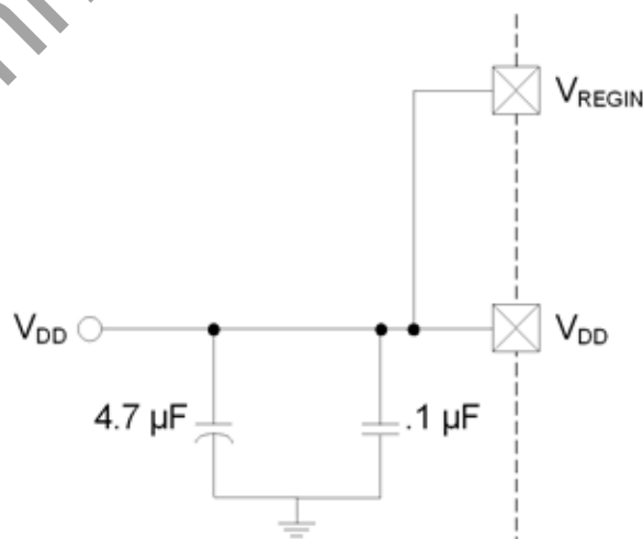
Figure 8.2. External Capacitors for Voltage Regulator Input/Output
