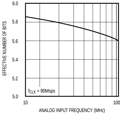
EFFECTIVE NUMBER OF BITS vs. ANALOG INPUT FREQUENCY
