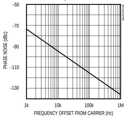
OSCILLATOR OPEN-LOOP PHASE NOISE vs. FREQUENCY OFFSET
