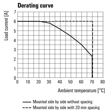
Derating curve
