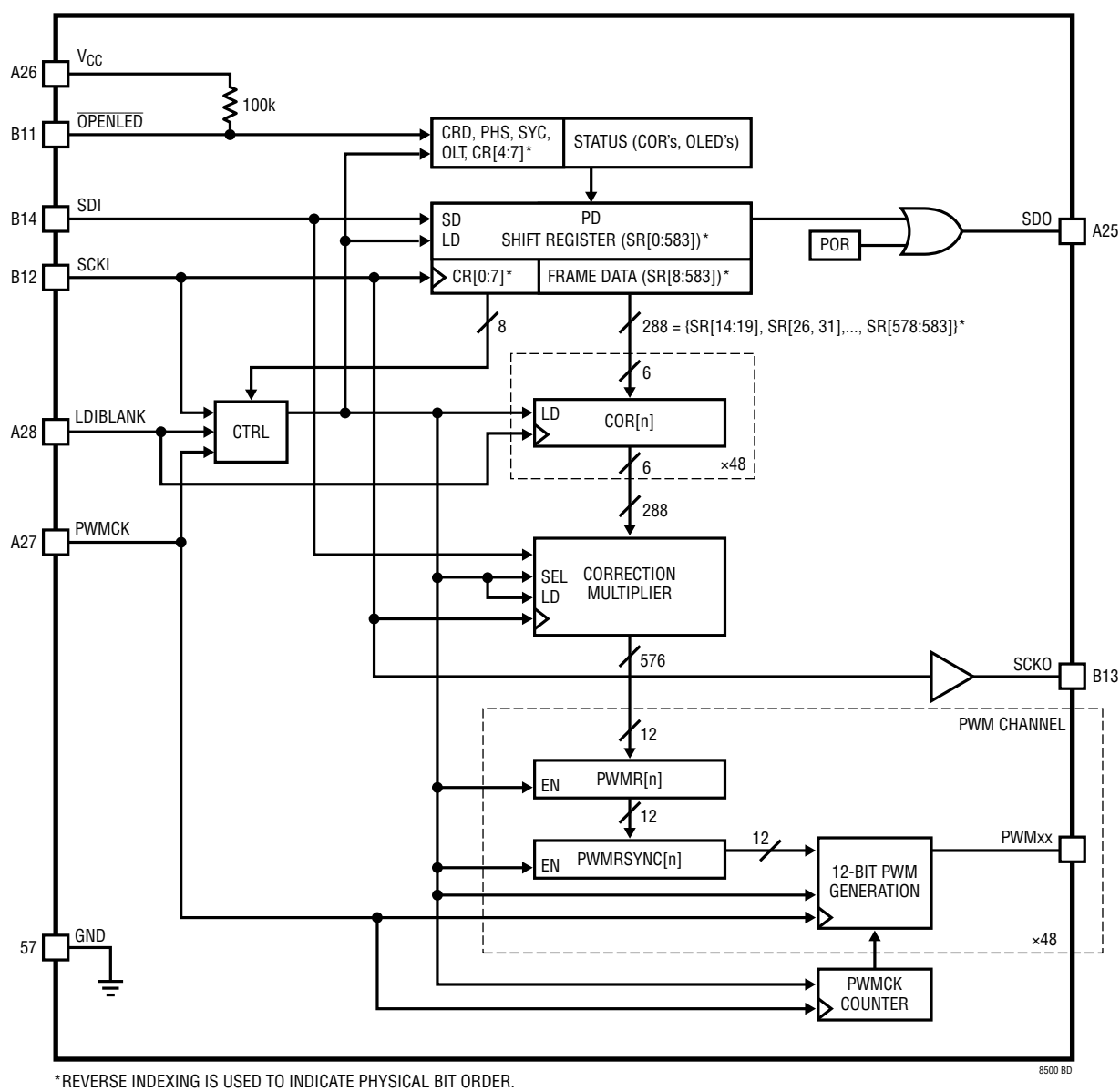
Figure 1. Block Diagram
