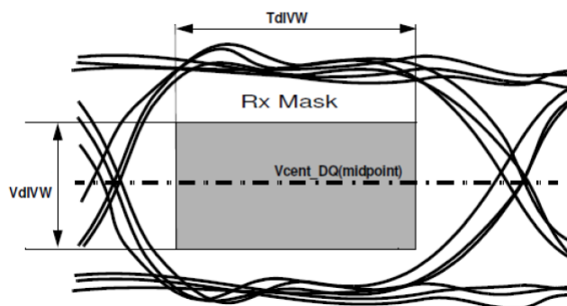
Figure 23. DQ Receiver(Rx) compliance mask
