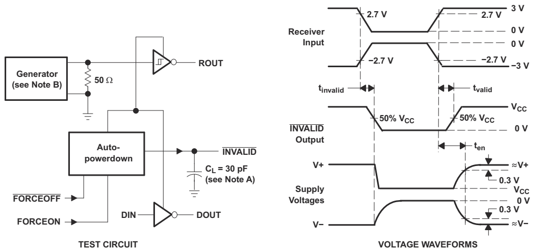
Figure 6-4. Receiver Enable and Disable Times
