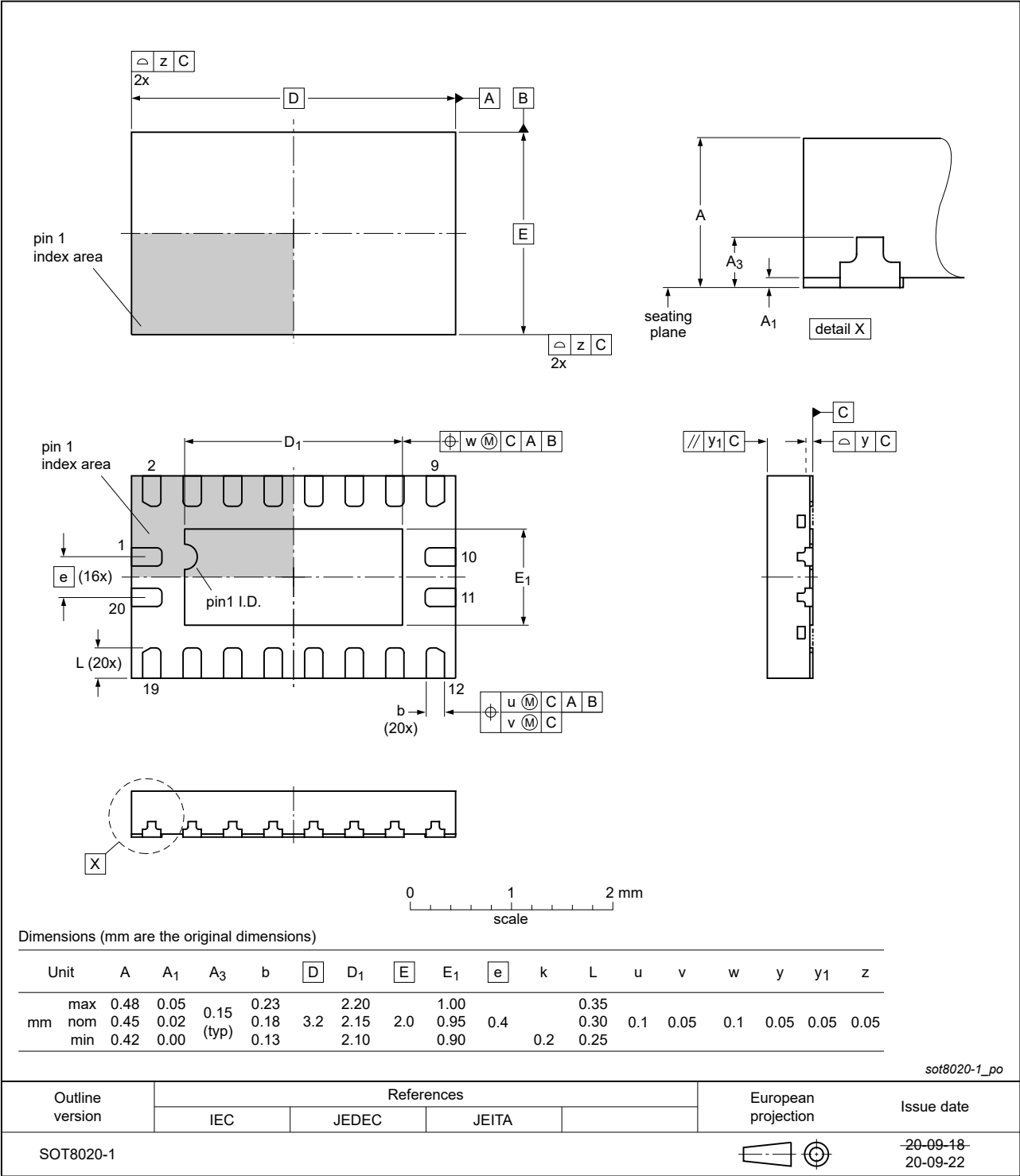
Fig. 14. Package outline SOT8020-1 (DHXQFN20)
