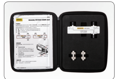
VSWR Bridge ( VB1020/VB1040 )
