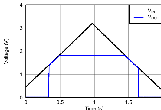
Figure 20. V_{IN} Power-Up and Power-Down
