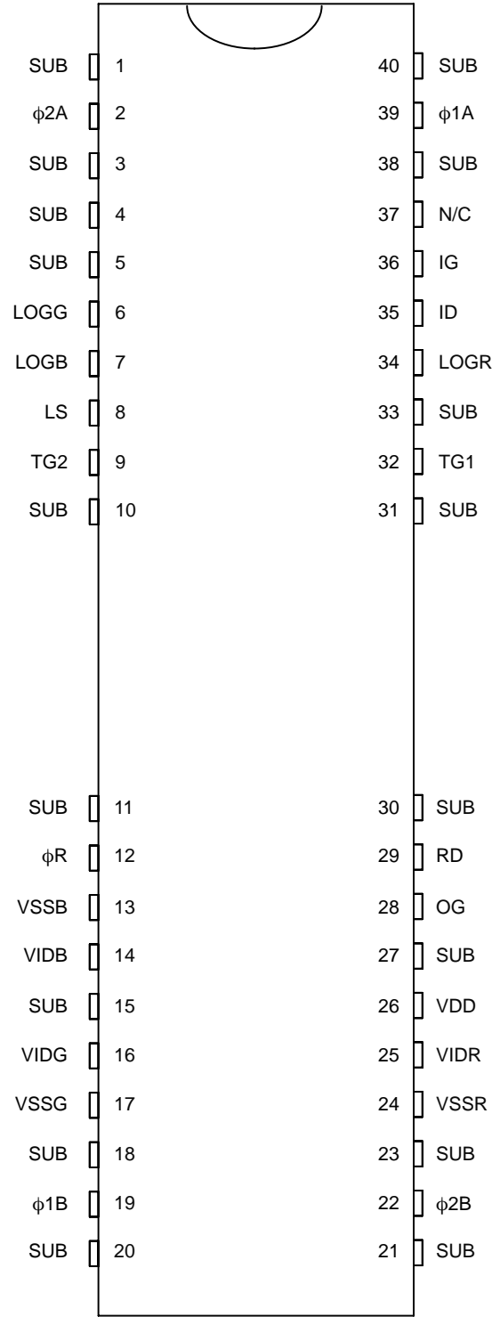
Figure 3. KLI-8023 Pinout
