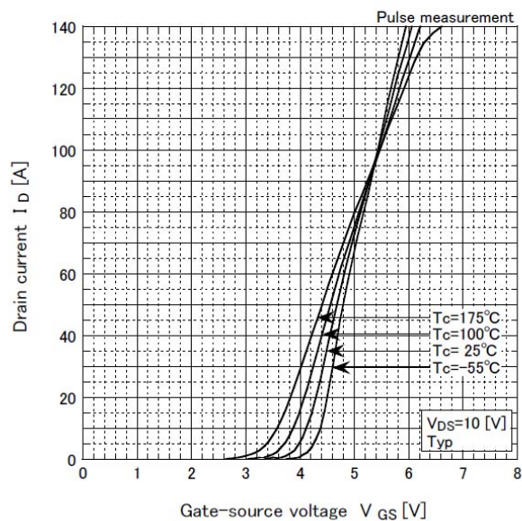
Transfer characteristics
