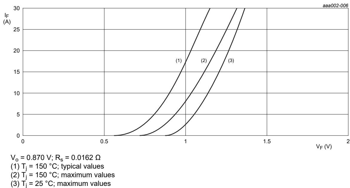
Fig. 6. Forward current as a function of forward voltage
