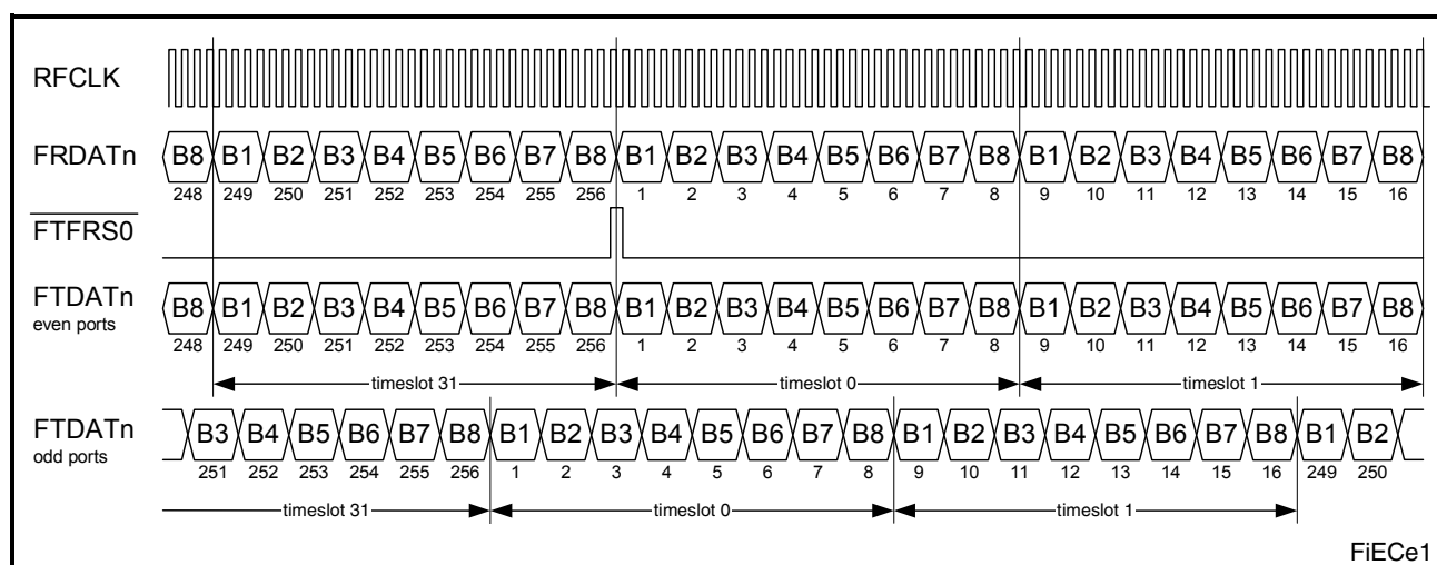
Figure 28 Framer Interface in EC Mode
