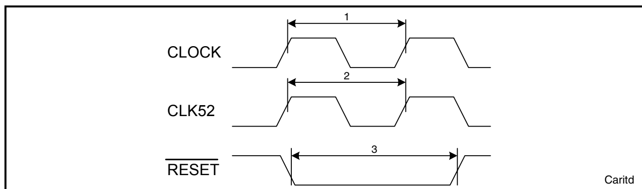
Figure 56 Clock and Reset Interface Timing Diagram
