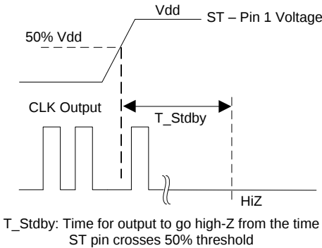
Figure 7. Standby Timing [5]
