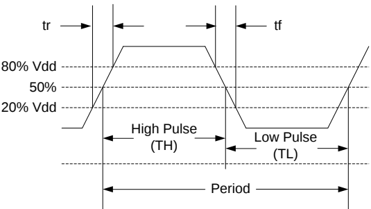
Figure 4. Waveform [4]
