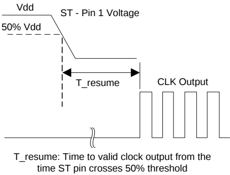
Figure 6. Resume Timing [5,6]
