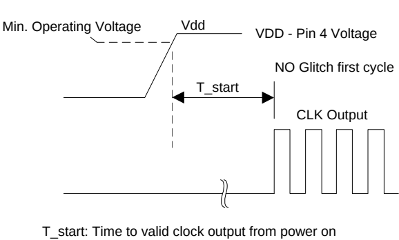
Figure 5. Startup Timing [5,6]
