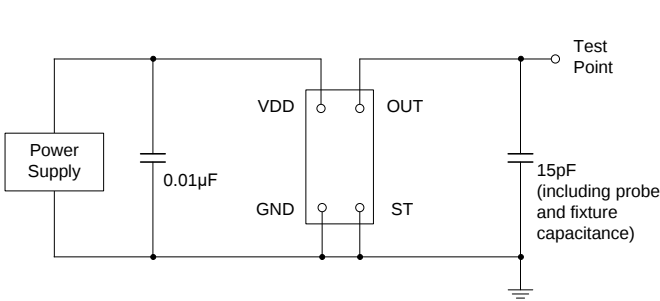
Figure 3. Test Circuit
