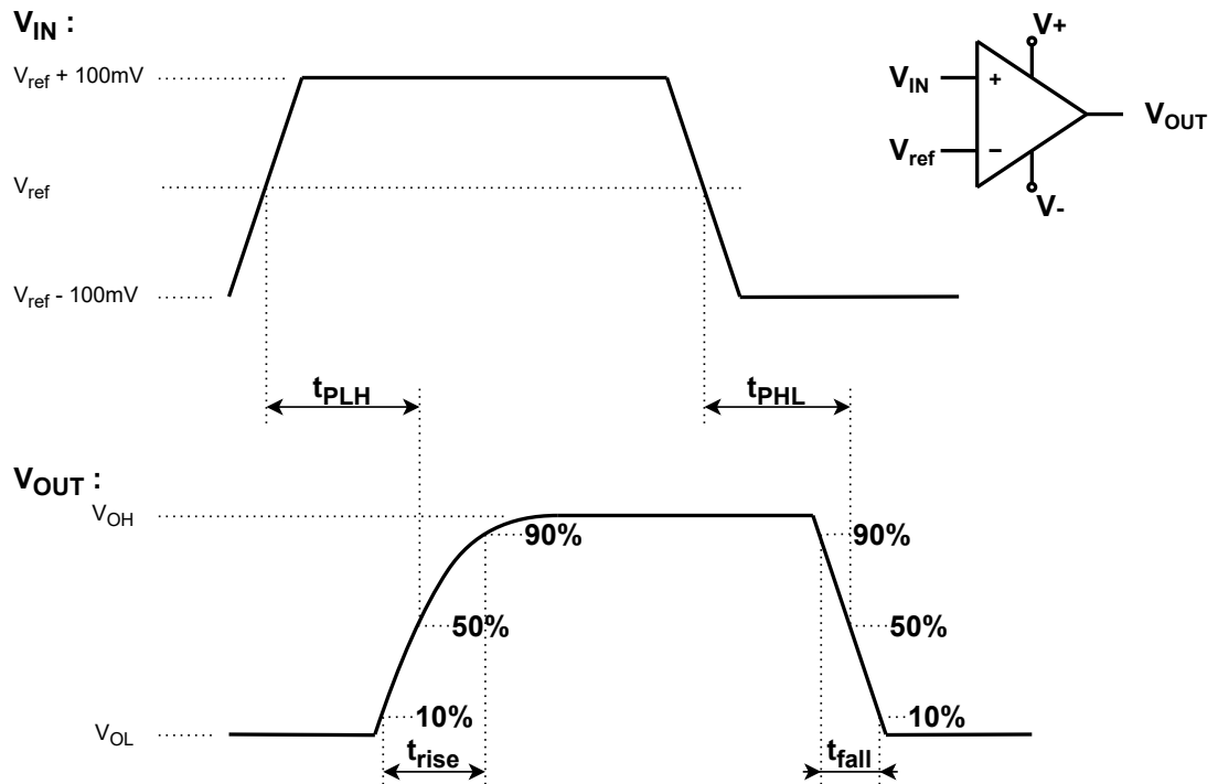
Figure 53. Propagation delay
