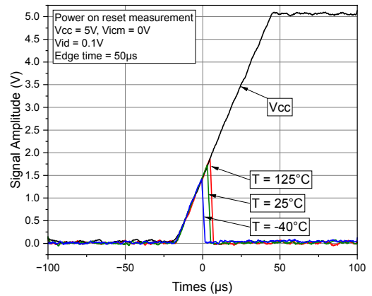
Figure 49. Power-on Reset output sequence V_{CC} = 5.0 V, R_{PU} = 2.5 k \Omega , V_{PU} = V_{CC}
