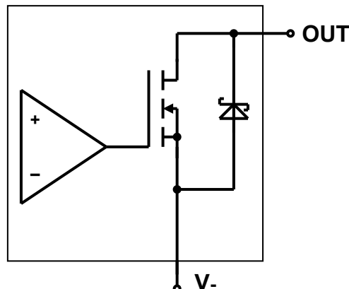
Figure 54. Output stage
