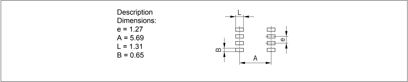
Figure 51 Footprint
