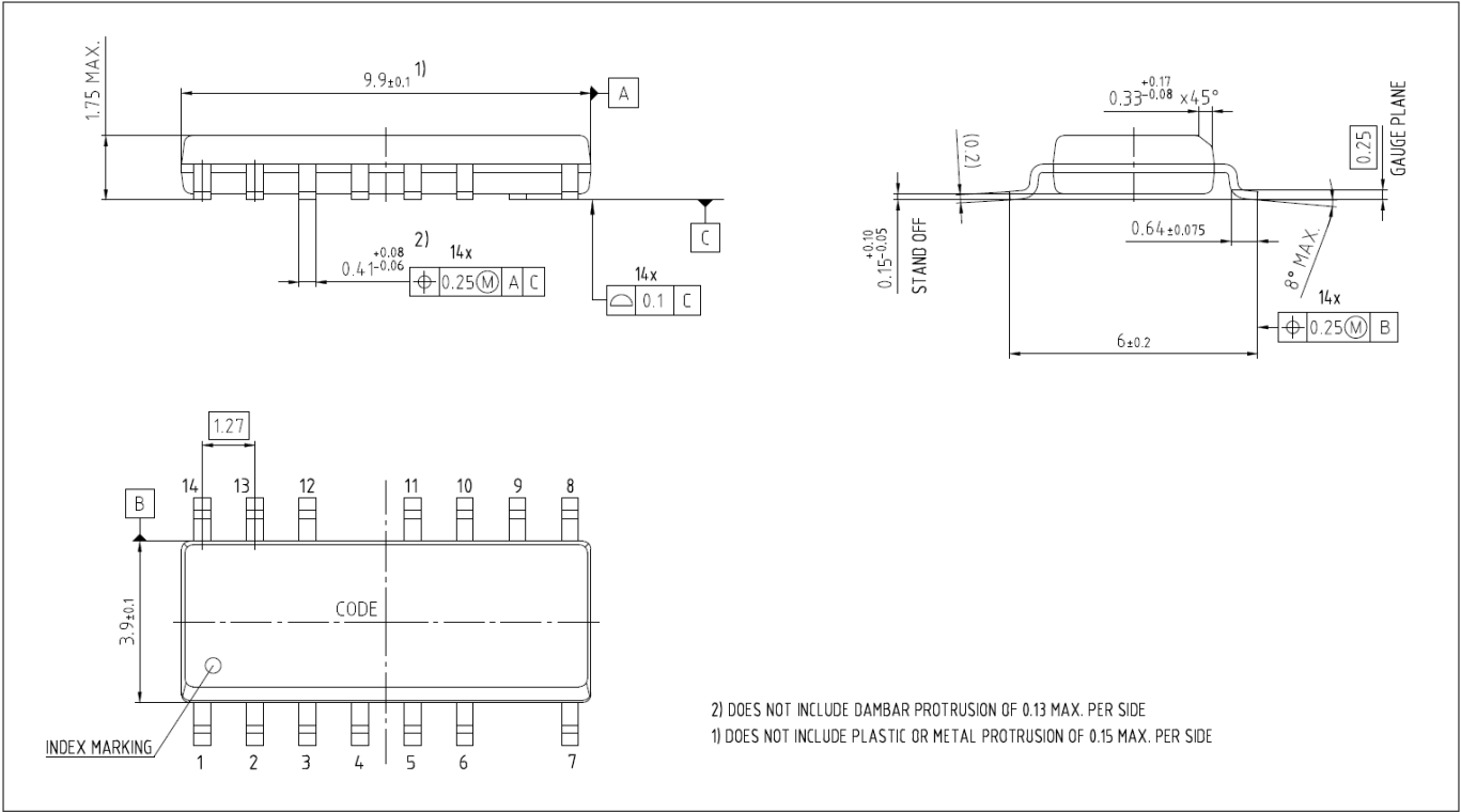
Figure 50 Outline
