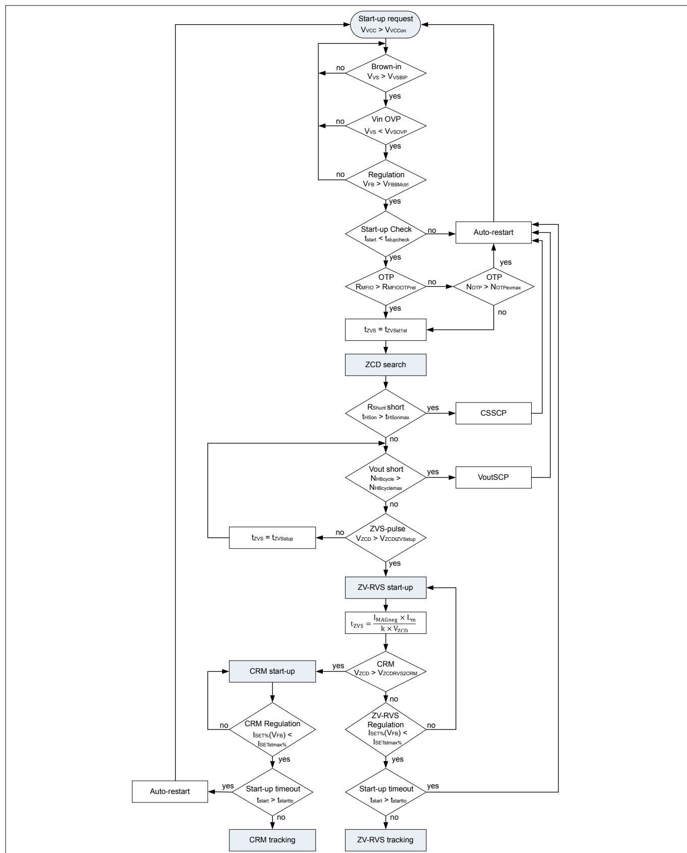
Figure 34 Start-up sequence
