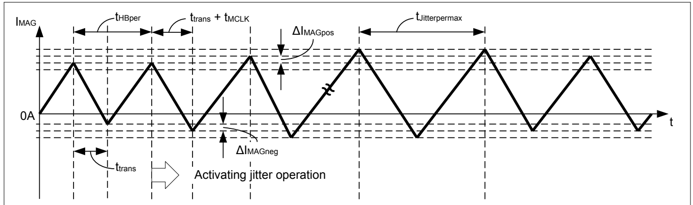
Figure 41 I_{\text{MAG}} modulation for frequency jittering
