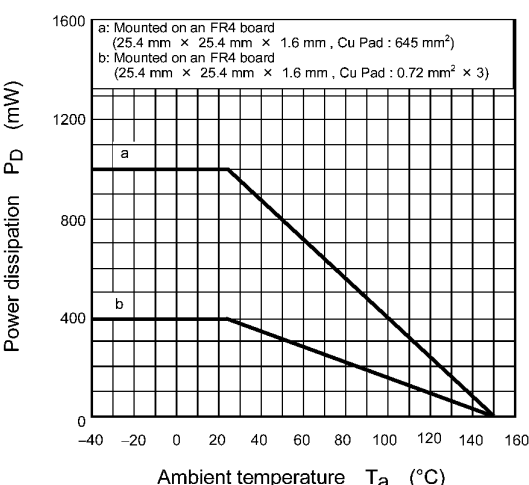
Fig. 8.12 P_D - T_a
