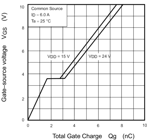
Fig. 8.10 Dynamic Input Characteristics
