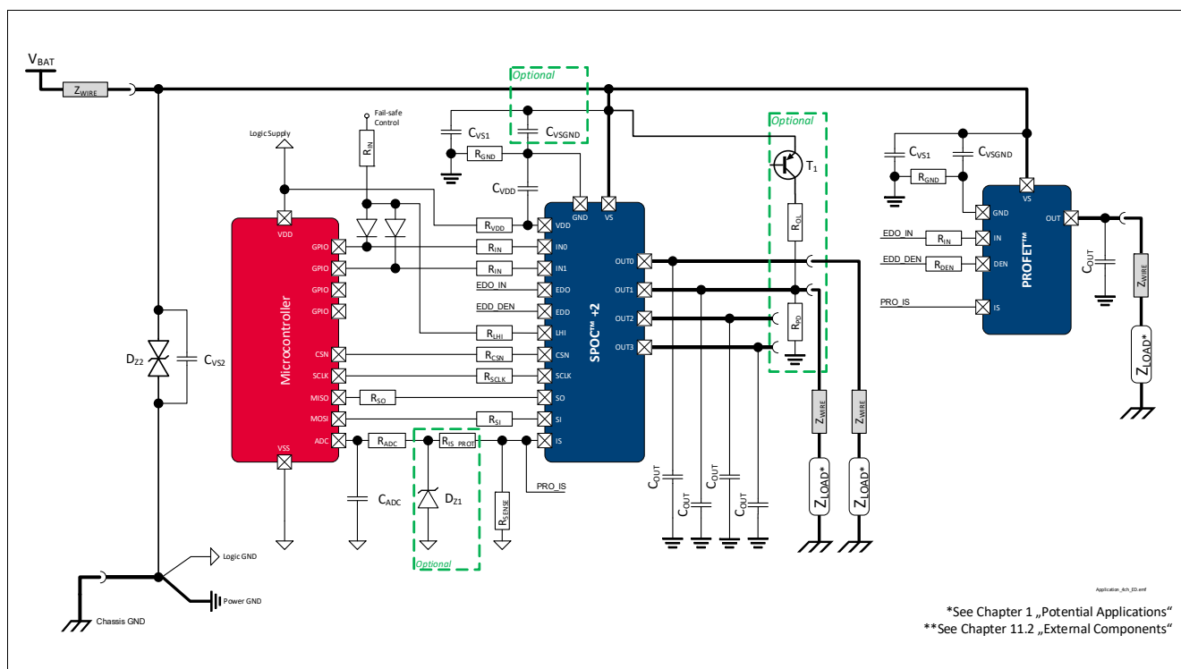
Figure 46 Application Diagram
