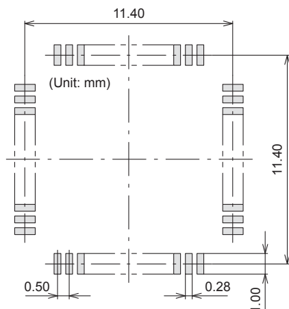
SOLDERING FOOTPRINT*
