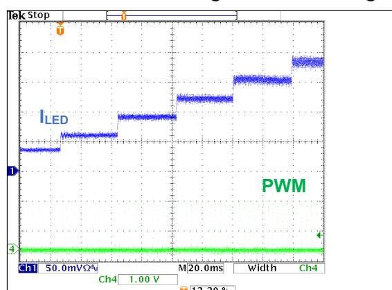
Reducing the visible change in LED luminance level by using C3
