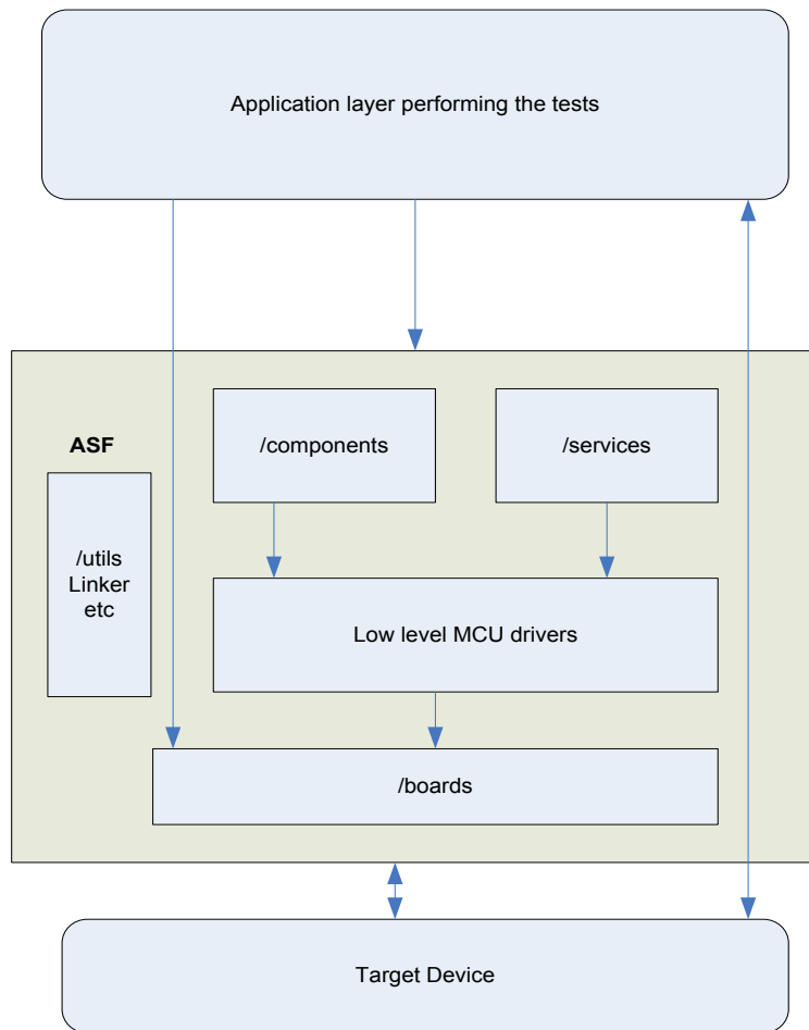
Figure 4-7. ASF Architecture
