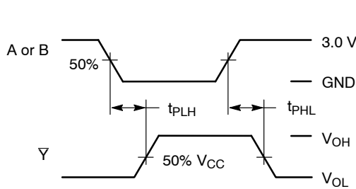
Figure 5. Switching Waveforms
