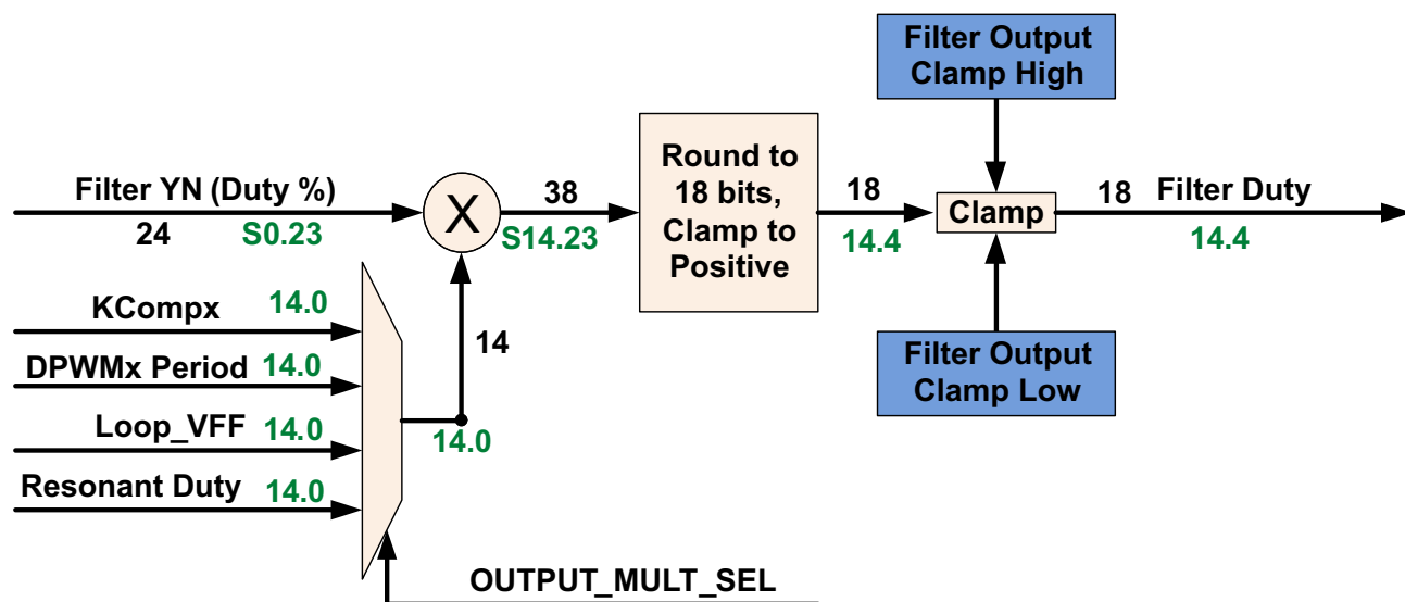
Figure 9-9. Resonant Mode
