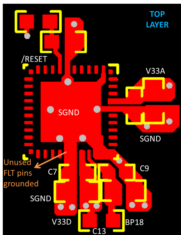
Figure 12-10. UCD3138 and UCD3138064 40 Pin Layout Top Layer
