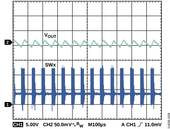
Figure 26. Steady State Waveform at Light Load, V_{IN} = 12\text{ V} , V_{OUT} = 3.3\text{ V} , I_{OUT} = 30\text{ mA} , f_{SW} = 600\text{ kHz} , L = 4.7\text{ μH} , C_{OUT} = 47\text{ μF} \times 2 , Automatic PWM/PSM Mode
