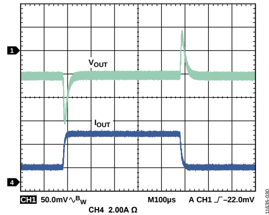
Figure 27. Channel 1/Channel 2 Load Transient, 1 A to 4 A, V_{IN} = 12\text{ V} , V_{OUT} = 3.3\text{ V} , f_{SW} = 600\text{ kHz} , L = 2.2\text{ μH} , C_{OUT} = 47\text{ μF} \times 2
