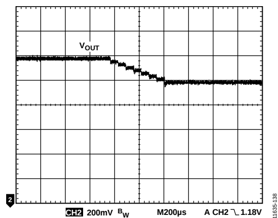
Figure 35. Channel 1 Dynamic Voltage Scaling (DVS) from 1.3 V to 1.1 V, 62.5 µs Interval, V_{IN} = 12 V, I_{OUT} = 4 A, f_{SW} = 600 kHz, L = 1 µH, C_{OUT} = 47 µF \times 2
