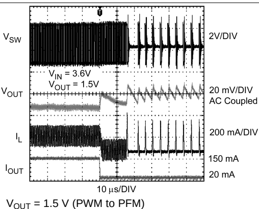
Figure 11. Mode Change by Load Transients
