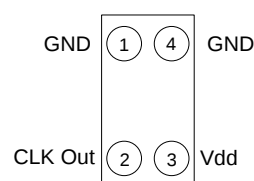
CSP Package (Top View)
