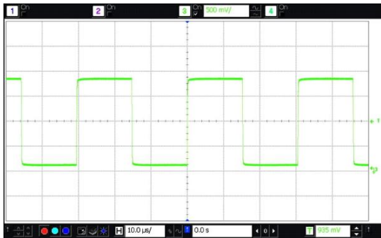
Figure 7. LVCMOS Waveform ( V_{dd} = 1.8\text{ V} ) into 15 pF Load
