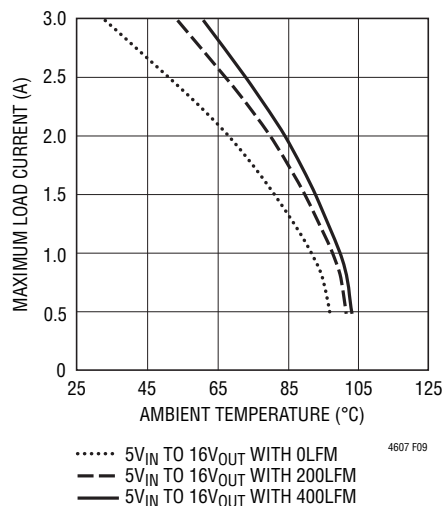
Figure 9. 5V IN to 16V OUT without Heat Sink
