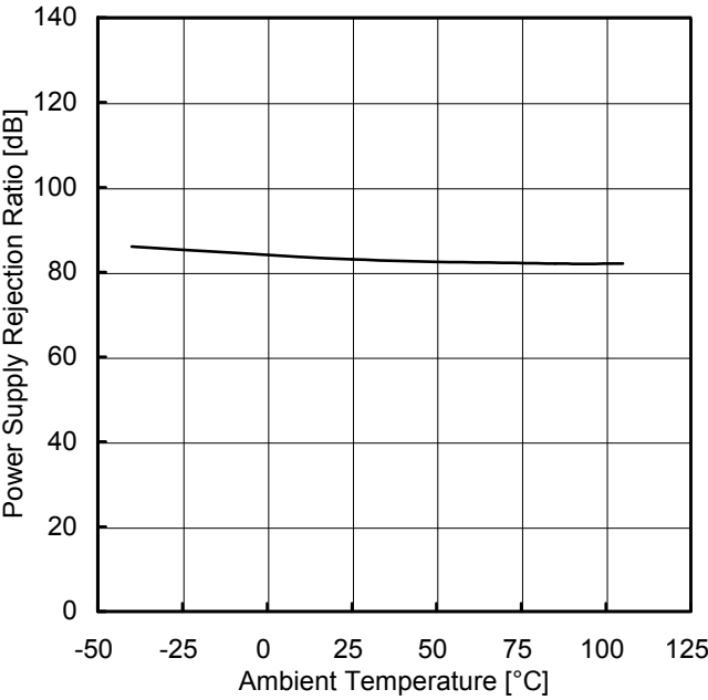
Figure 44. Power Supply Rejection Ratio vs Ambient Temperature
