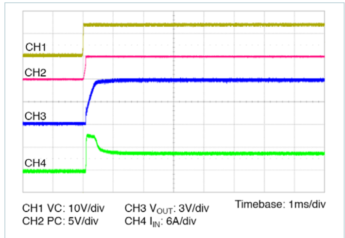
Figure 14 — Start up from application of VC; V_{IN} pre-applied C_{OUT} = 4000\mu F
