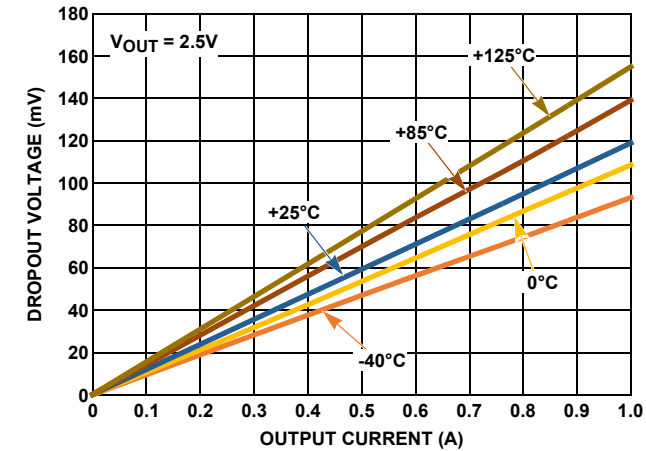
FIGURE 4. DROPOUT vs OUTPUT CURRENT
