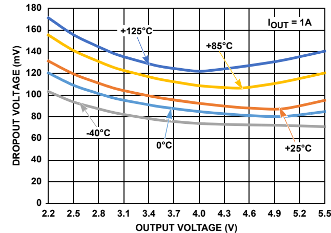
FIGURE 6. DROPOUT vs OUTPUT VOLTAGE
