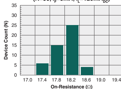
Typical On-Resistance Distribution (N=50, I_F=5\text{mA} , I_L=120\text{mA}_{DC} )
