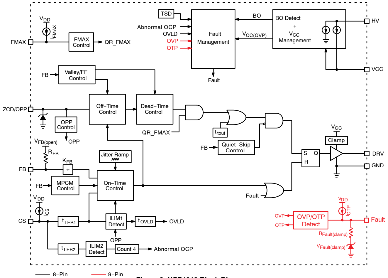
Figure 3. NCP1343 Block Diagram
