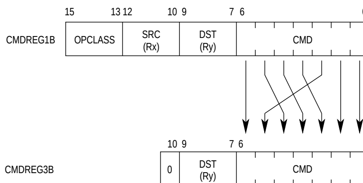
Figure 9-11. Mapping of Command Bits for CMDREG3B Field
