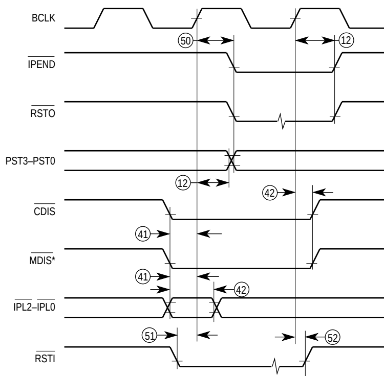
Figure C-17. Other Signal Timing
