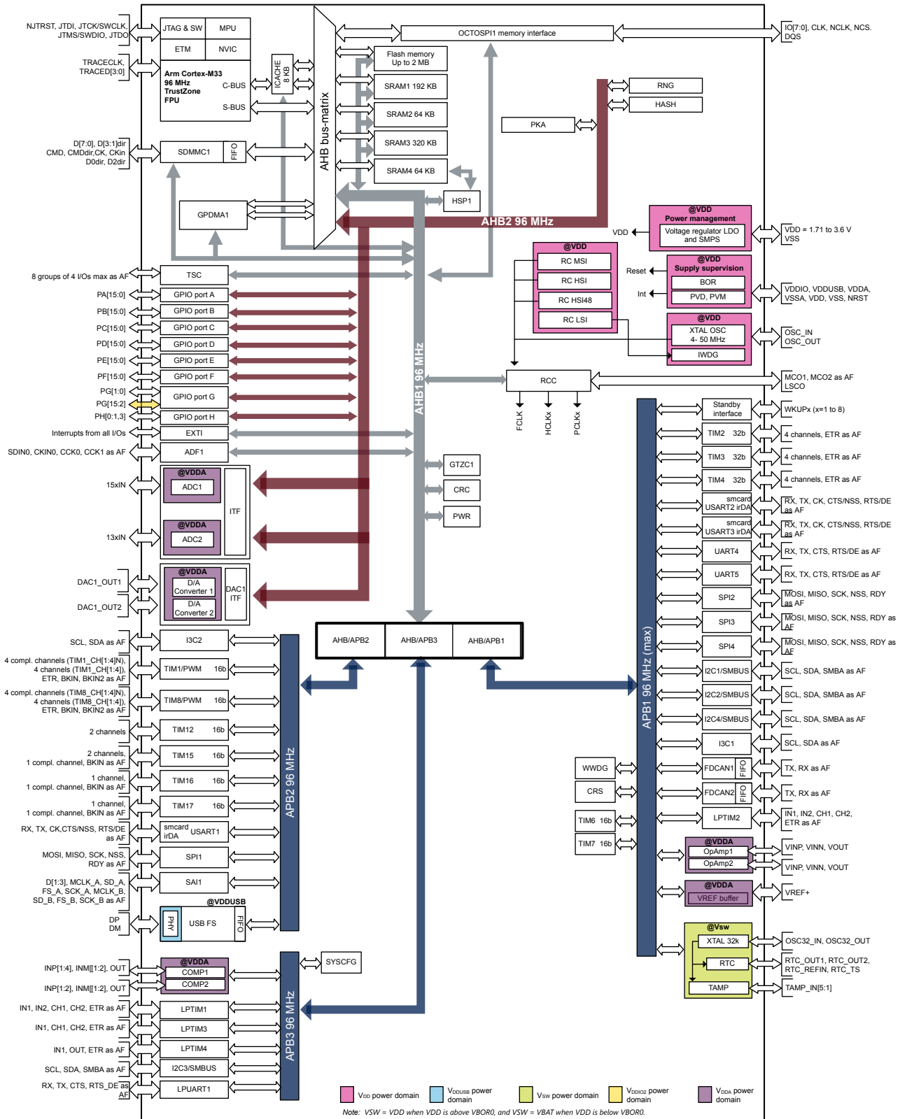
Figure 1. STM32U3B5xx block diagram
