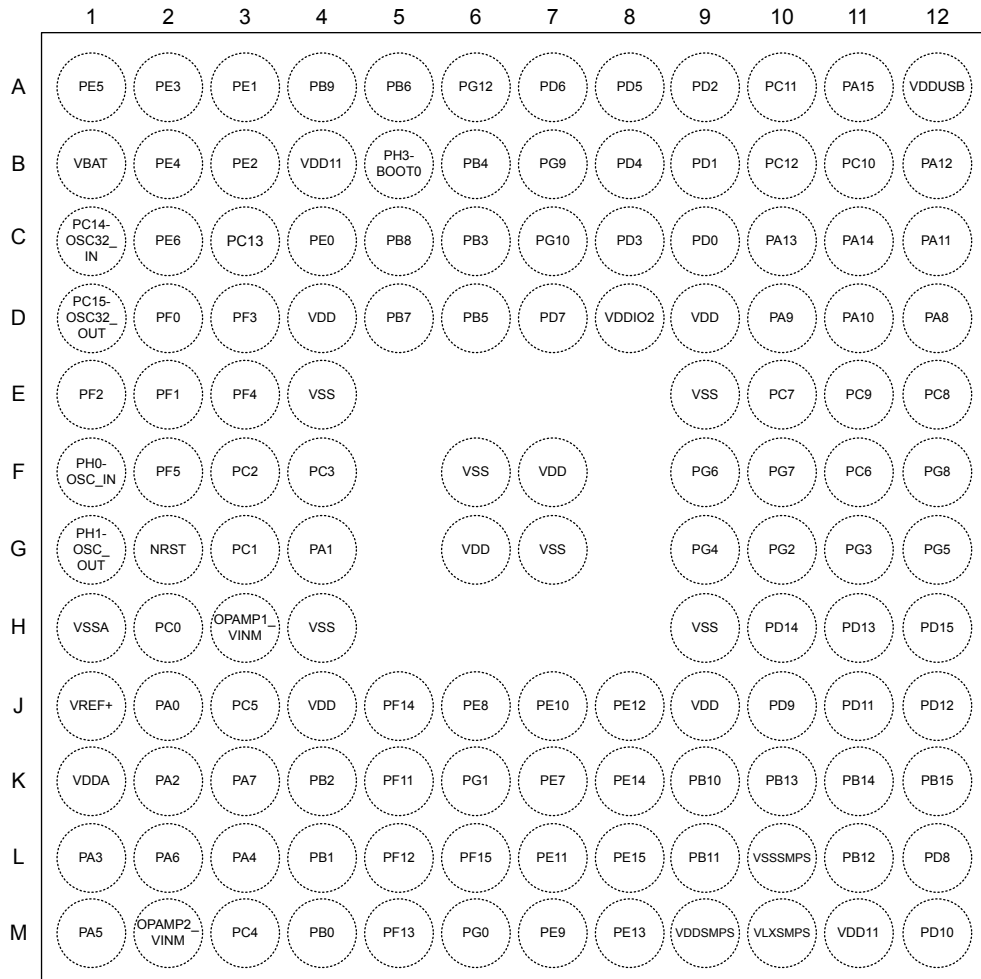
Figure 17. UFBGA132_SMPS ballout
