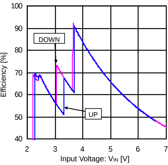
Figure 3. Efficiency Hysteresis vs Input Voltage (13mA x 6 Lights)
