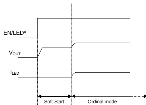
Figure 14. Soft-Start
