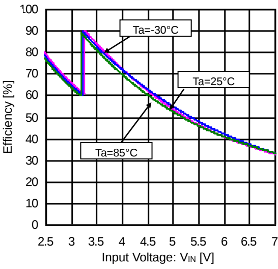
Figure 4. Efficiency vs Input Voltage (3.5mA x 6 Lights)
