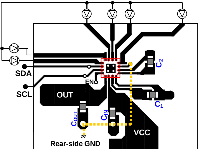
Figure 16. Front (Top View)
