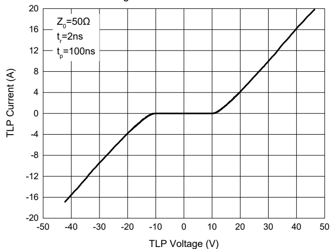
Fig. 5 - TLP Measurement
