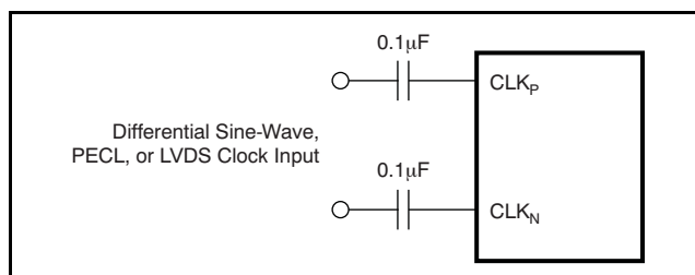
Figure 37. Differential Clock Driving Circuit (DIFF_CLK = 1)
