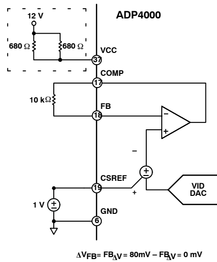
Figure 6. Positioning Voltage
