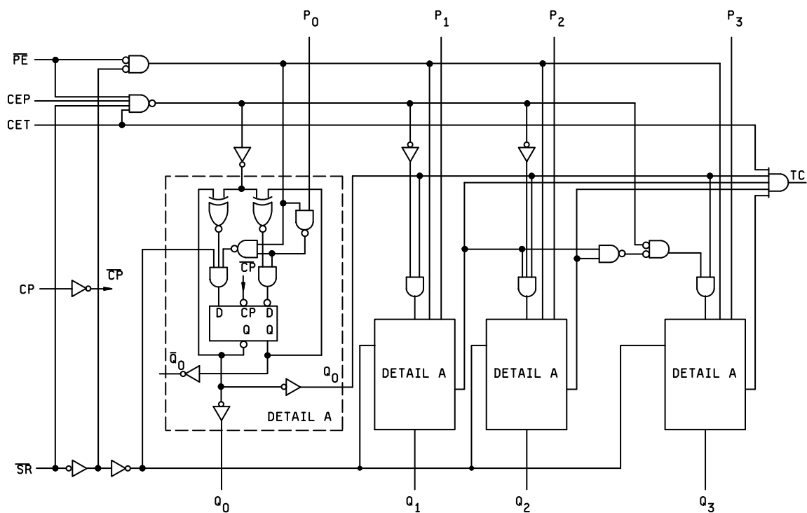
FIGURE 3. Logic diagram.
