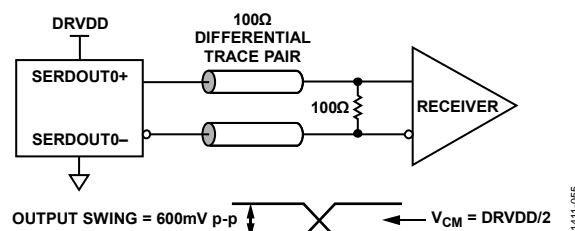
Figure 55. DC-Coupled Digital Output Termination Example
