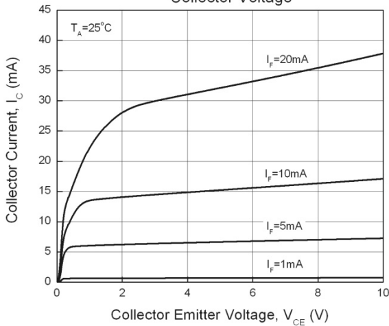
Figure 5. Collector Current vs Collector Voltage
