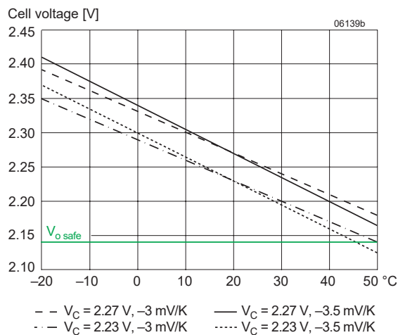
Fig. 12 Trickle charge voltage versus temperature for defined temperature coefficient. V_{o \text{ nom}} is the output voltage with open R-input.
