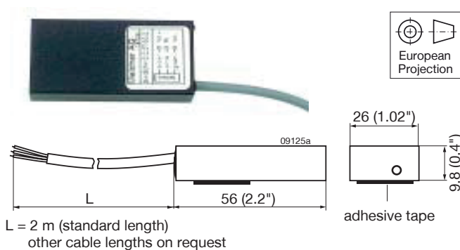
Fig. 30 Battery temperature sensor
